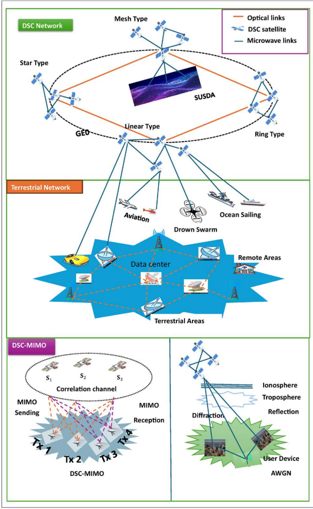
Fig. 2: Architecture of SUSDA satellite-ground collaborative transmission [9]
