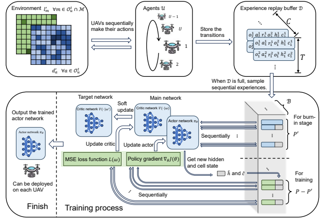
Figure 1: Our training framework.
