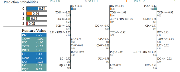
Fig. 2. \hat{x} AI Module results highlighting the parameters governing the EQAI-VQC decision to determine the authenticity of a received message by vehicles.
