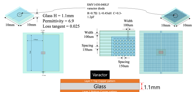
Fig 1. Unitcell structure
