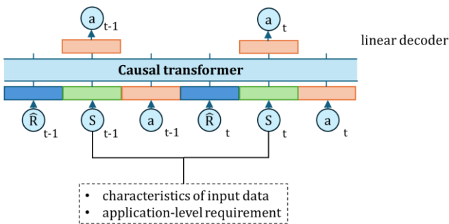
Fig. 1. Decision transformer Architecture
