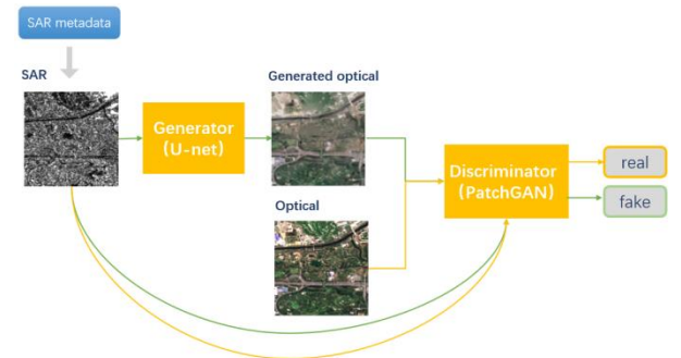
Figure 1. cGAN model for S2O image conversion
