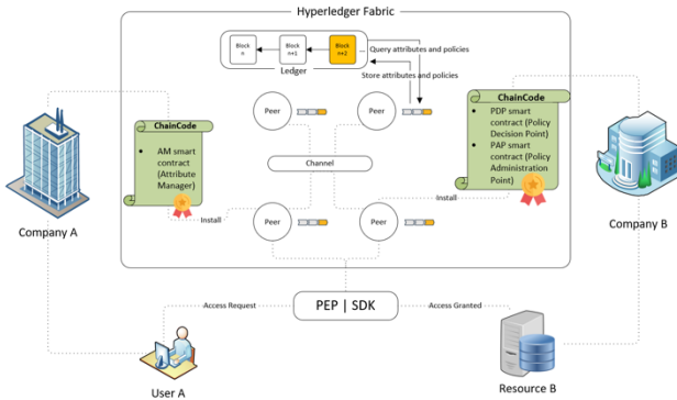
Figure 2. Proposed architecture
