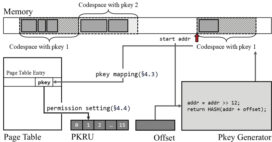
Fig. 2. Protecting Codespace with Intel MPK
