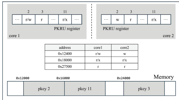
Fig. 1. How Intel MPK Works
