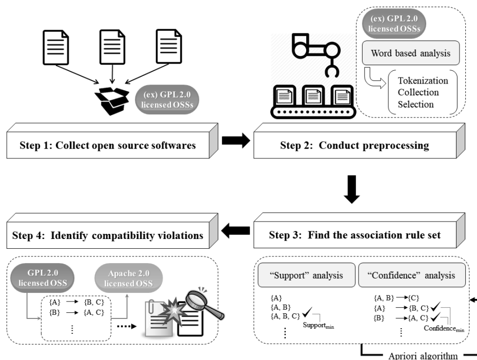
Fig. 3. Overall Approach
