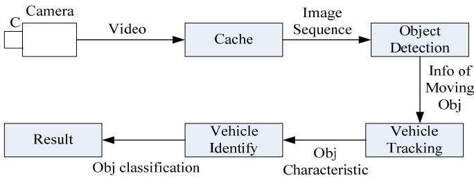
Fig. 1. Flow chart of the video traffic flow detection system.
