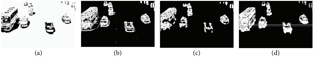
Fig. 8. The processes of elimination of moving cast shadows: (a) the pre-extraction of the cast shadows, (b) the binary edge image, (c) the elimination of the cast shadows edge pixels, and (d) the binary image of object areas.
